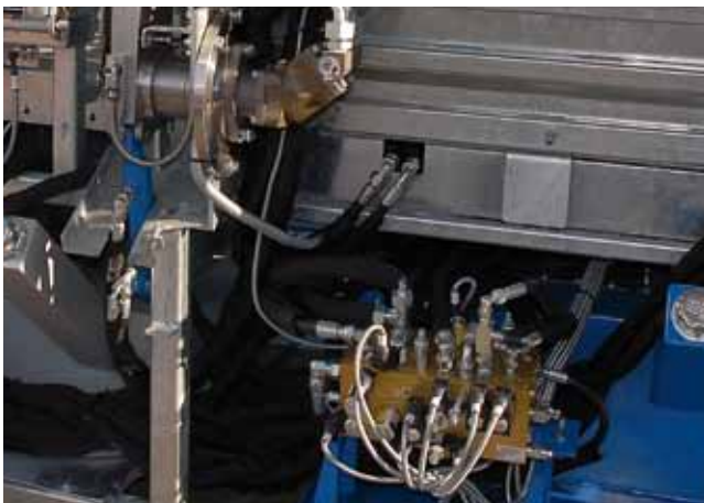
Links: Sägeaggregat, rechts: Kompakter Ventilblock
